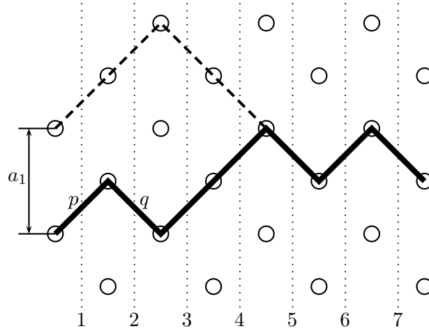
Figure 8.2: The thick, full line shows the configuration of the lattice after an avalanche has passed through. Each up or down-pointing segment corresponds to a single site, the position label of which is shown under the dotted line. A segment pointing upwards corresponds to a site being in state z = 1 (with probability p , see Eq. (8.28b)), a segment pointing downwards corresponds to state z = 2 (probability q ), as indicated. The dashed line corresponds to a “toppling trajectory” as explained in the text.
