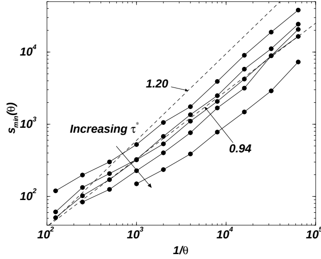
Figure 4.21: The position of the minimum in the binned and rescaled histogram for different values of \tau^* = 2.04, 2.08, 2.10, 2.12, 2.16 . The exponents shown in the plot are for comparison only.
