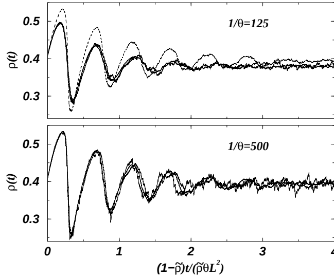
Figure 4.36: The density of trees as a function of time, plotted versus the rescaled time (1 - \bar{\rho})t/(\bar{\rho}\bar{\theta}L^2) . Upper panel: Plot for \theta^{-1} = 125 and L = 1000, 2000, 4000 with an additional plot for \theta^{-1} = 500 and L = 4000 shown as dashed line, for comparison of period and amplitude. Lower panel: Same plot for \theta^{-1} = 500 and L = 1000, 2000, 4000 .
