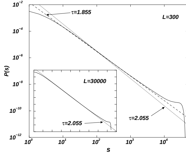
Figure 2.6: Cluster size distribution \mathcal{P}(s) for site percolation with L = 300 (main panel) and L = 30000 (inset). Neither of these systems should be considered as particularly small. However, the best estimate for the intermediate slope of \mathcal{P}(s) for L = 300 in a double logarithmic plot, is, as shown as a dashed line, \tau = 1.855 which is 10% off the correct value \tau \approx 2.055 shown as a dotted line. In the inset, the correct exponent is shown to fit fairly good the intermediate slope of the data for L = 30000 .
