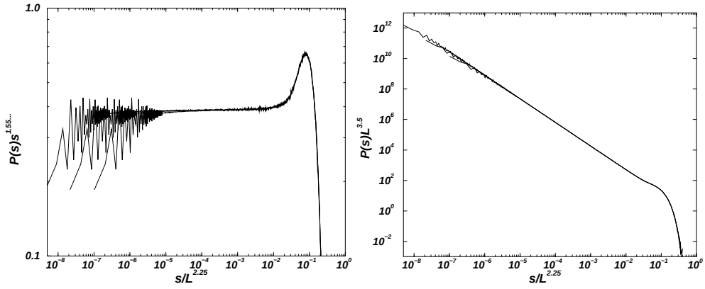
Figure 2.4: Comparison of different ways of collapsing data which follows simple scaling in a double logarithmic plot. The data is taken from the original Oslo model, where s is the avalanche size. The left plot shows \mathcal{P}(s)s^\tau versus s/L^D , the right one \mathcal{P}(s)L^{D\tau} versus the same s/L^D . Due to the continuous decrease, the right plot cannot show as much details as the left. Data are taken from the original Oslo model with L = 1280, 2560, 5120 , and exponents \tau = 1.555\dots and D = 2.25 , i.e. the PDF scales like \mathcal{P}(s) = as^{-\tau}\mathcal{G}(s/(bL^D)) .
