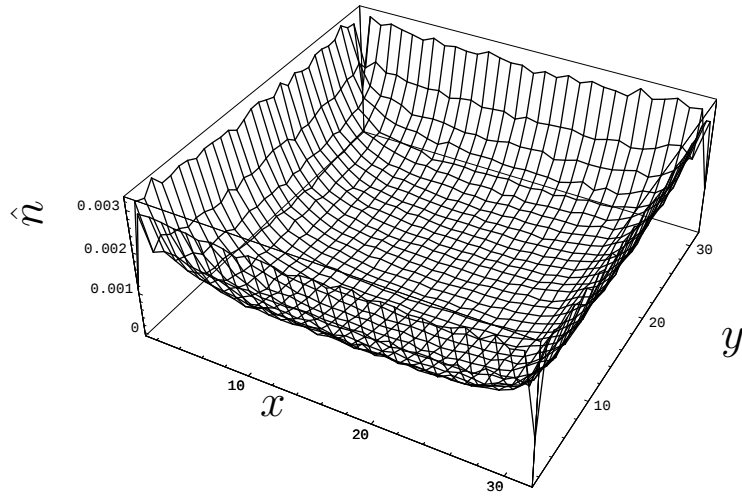
Figure 3.3: Average number \hat{n} of times a site was the seed of an avalanche in the OFC model, i.e. probability to be seed per site. Simulation parameters: L = 32 , open boundaries, \alpha = 0.24 , 2 \times 10^5 avalanches for transient and 5 \times 10^5 for statistics.
