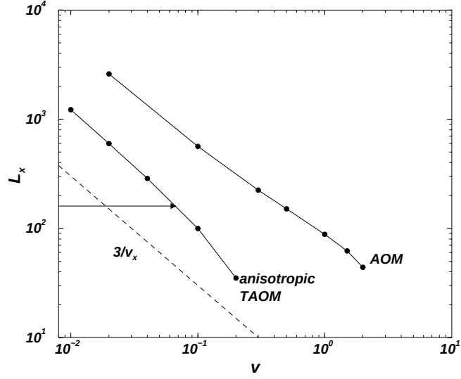
Figure 7.11: Scaling of the crossover system size versus the anisotropy v_x in the anisotropic TAOM (see Fig. 7.7(a), page 280) and the AOM (Fig. 7.2, page 275). The dashed line corresponds to (7.67). The horizontal arrow marks the crossing velocity for L = 160 , which is shown as arrow in Fig. 7.10 and Fig. 7.12.
