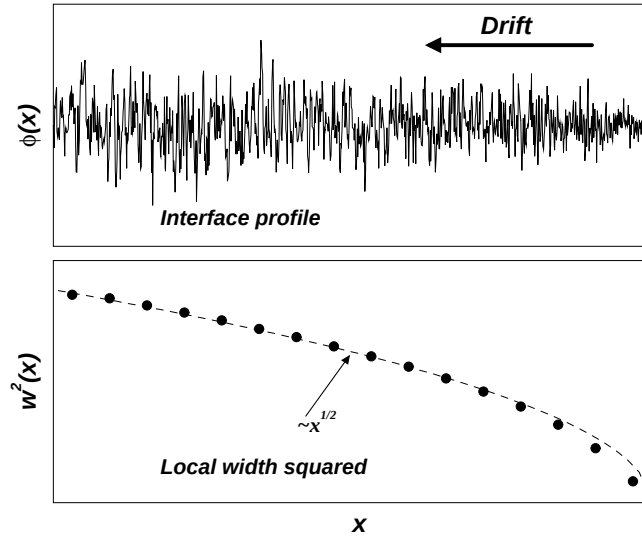
Figure 9.2: A qualitative picture of an interface snapshot with its “local roughness”; scales are irrelevant. Upper panel: An example of an interface profile with fixed boundaries and drift term. Lower panel: The ensemble averaged local width squared (numerical data, circles) is proportional to the square root of the position where measured, (L - x)^{1/2} (fitted, dashed line).
