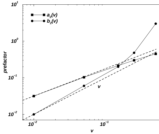
Figure 7.14: Scaling of the two sets of parameters used in the inset of Fig. 7.13 to force a data collapse. The parameters seem to scale nicely for sufficiently small v , as indicated by the two thick dashed lines.
