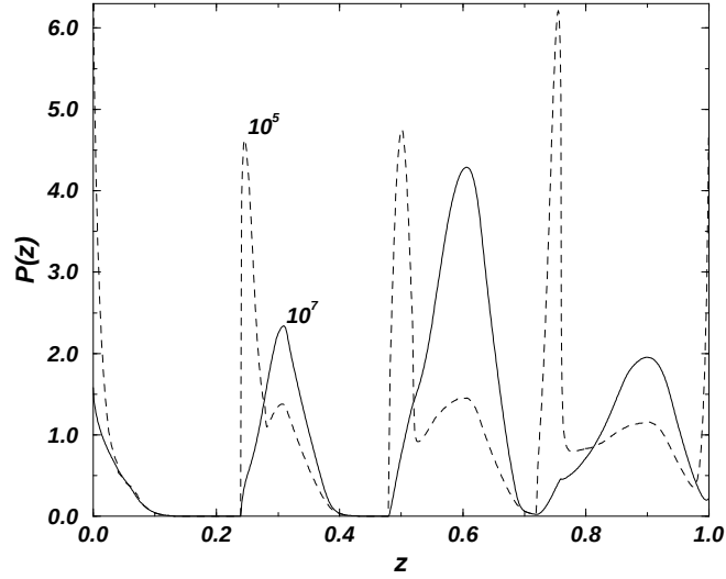
Figure 3.1: Height distribution in the two dimensional OFC model on a square lattice for L = 256 , open boundaries and \alpha = 0.24 after 10 \times 10^6 avalanches, averaged over 10^6 avalanches. The four bumps correspond to four charges of a site. There is a general problem of slow convergence in the OFC model (not discussed here), which is illustrated by the distribution after 10^5 avalanches (averaged over the same number) shown as a dashed line.
