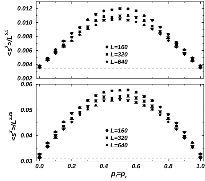
Figure 7.6: The rescaled second and third moments, \langle s^2 \rangle / L^{3.25} and \langle s^3 \rangle / L^{5.5} , of the anisotropic OOM in the isotropic regime for various different values for p_r = p_l , and L = 160, 320, 640 . The small variation of the ratio in L is probably only due to finite size effects. The straight dashed line indicates the amplitude found in the OOM.
