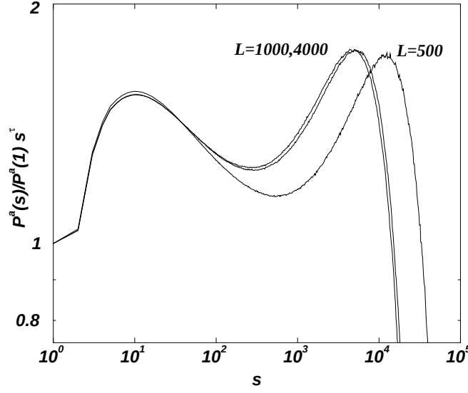
Figure 4.27: Plot of the rescaled PDF \mathcal{P}^a(s; \theta, L) s^{\tau^*} / \mathcal{P}^a(1; \theta, L) for fixed \bar{\rho} \approx 0.397 : L = 500 with 1/\theta = 2000 ( \bar{\rho} = 0.396827 ), L = 1000 with 1/\theta = 940 ( \bar{\rho} = 0.396825 ) and L = 4000 with 1/\theta = 870 ( \bar{\rho} = 0.396883 ). Again, a data collapse is impossible.
