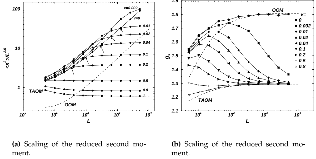
Figure 7.7: Scaling in the in the anisotropic TAOM . Fig. 7.7(a): Rescaled second moment \langle s^2 \rangle / L^{2.5} in the anisotropic TAOM versus L for various values of \nu . For larger \nu the TAOM behaviour is observed much earlier. At \nu = 1 the anisotropic TAOM is identical to the TAOM. The dashed lines are for the corresponding data of the OOM and the TAOM. The line for \nu = 0 runs parallel to the OOM data. The arrows show the estimated crossover as shown in Fig. 7.11. Fig. 7.7(b): Moment ratio g_3 in the anisotropic TAOM for different \nu as indicated, The smaller \nu the later the crossover to the TAOM sets in.
