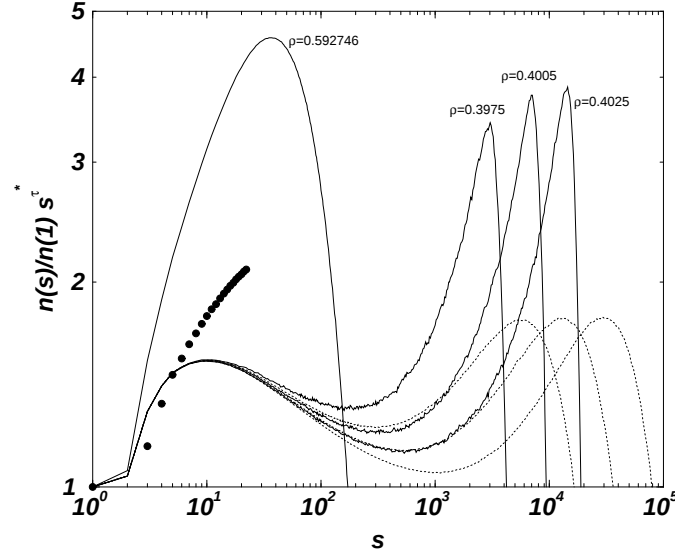
Figure 4.24: The rescaled and binned histogram \bar{n}(s; \rho) s^{\tau^*} (again \tau^* = 2.10 ), for a modified model, where the largest cluster in the system is removed in each relaxation step and the corresponding number of trees is filled back into the system afterwards. The three small values of \rho chosen, \rho = 0.3975, 0.4005, 0.4025 correspond (up to the last digit) to the values of the tree density for \theta^{-1} = 1000, 2000, 4000 respectively, see Tab. 4.3. The linear size was L = 1000, 2000, 4000 . The corresponding data of the original model are shown dotted. The peculiar behaviour of the different height-scaling of the minimum and the maximum is again visible (a correct tilt \tau^* would make it even more pronounced), but disappears obviously for \rho = \rho_{\text{perc}} – for these data it is relevant to mention that \bar{n}(s) was measured after the relaxation. The filled circles show the exact results for the lattice animals (Stauffer and Aharony, 1994; Sykes and Glen, 1976; Mertens, 1990) at \rho = \rho_{\text{perc}} .
