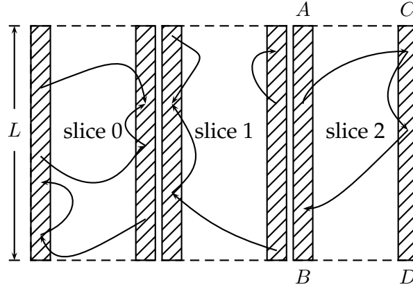
Figure 4.15: The slices, three of which are shown here, maintain the references for all clusters within each slice (illustrated by arrows), even for border clusters. The references between slices, however, are maintained by the master. The variables A = 0 , B=L-1 , C = I and D = I + L - 1 are the indices used for references within each slice.
