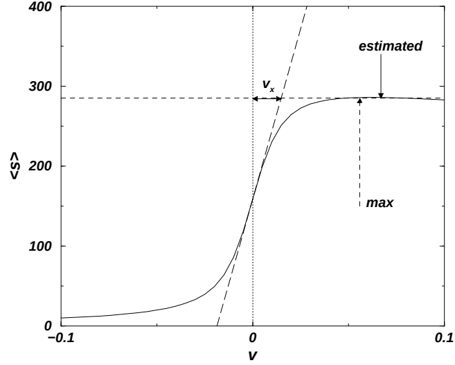
Figure 7.12: Equation (7.56) for L = 160 , as already shown in Fig. 7.10. The asymptotic maximum average avalanche size is marked by a dashed horizontal line, the dashed arrow indicates the position of this maximum, see (7.63b). The long dashed line is (7.66) and the double arrow is \nu_x derived from this equation. The arrow from top (labelled “estimated”) is the estimate for the crossover velocity as derived from Fig. 7.11.
