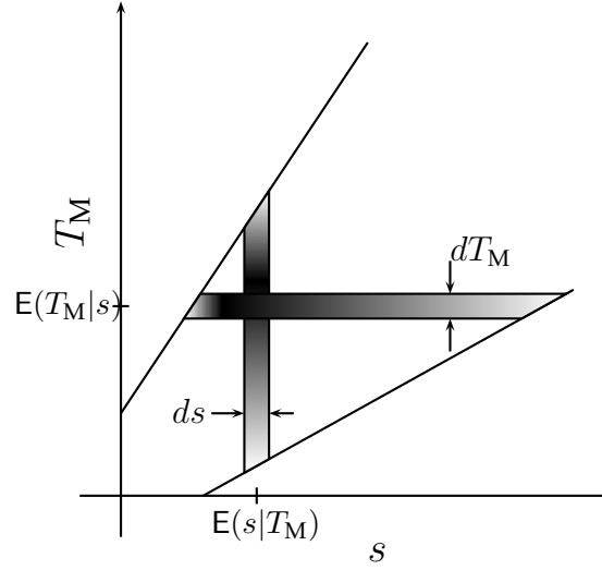
Figure 4.4: A schematic joint PDF P(s, T_M'; \theta) . The gray shading is used to indicate the density and the straight lines indicate roughly the limits of the distribution. While a narrower distribution would most easily obey (4.18), it does not necessarily have to be sharply peaked. In this example the weighted areas of the horizontal and the vertical stripes might be the same. They cross at the conditional averages.
