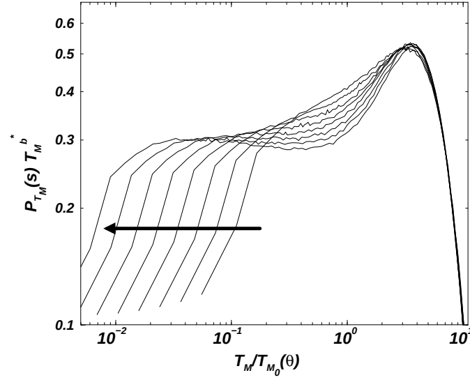
Figure 4.33: Attempt of a data collapse for P_{T_M}(T_M; \theta) . Only at the far end of the scaling function at the descent from the maximum, the data seem actually to collapse. This, however, is not sufficient for a data collapse. The big arrow points in the direction of increasing \theta^{-1} .
