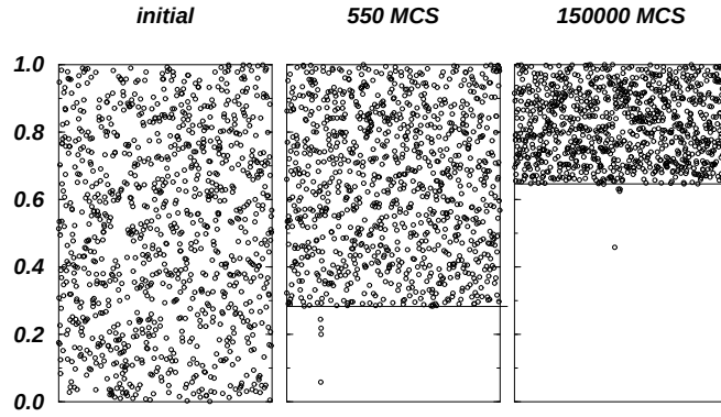
Figure 1.8: The configuration for a system of size N = 1000 after three different t . Typically only a few number of sites are active (below g(t) ) and even less for early t . The value of the gap function is indicated by a straight line.
