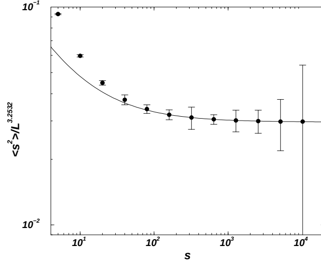
Figure 2.10: The rescaled second moment \langle s^2 \rangle / L^{\gamma_2} of the avalanche size distribution of the original Oslo model as a function of the system size L . The full line is based on a (four-parameter) fit of the data in the range L \in [40, \dots, 10240] against (2.58) with one correction; \langle s^2 \rangle = c_0 L_2^\gamma + c_1 M_0^{\gamma_2 - \omega_1} .
