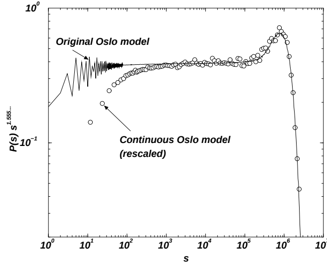
Figure 2.3: Comparison of the scaling function of the original and the continuous Oslo model (see chapter 5). The scaling function is obtained by multiplying the PDF (distribution of the avalanche sizes s ) by an appropriate power of s , in this case \tau = 1.555 \dots . One can clearly see the onset of the actual scaling behaviour and the presumably non-universal behaviour of the distribution below the lower cutoff.
