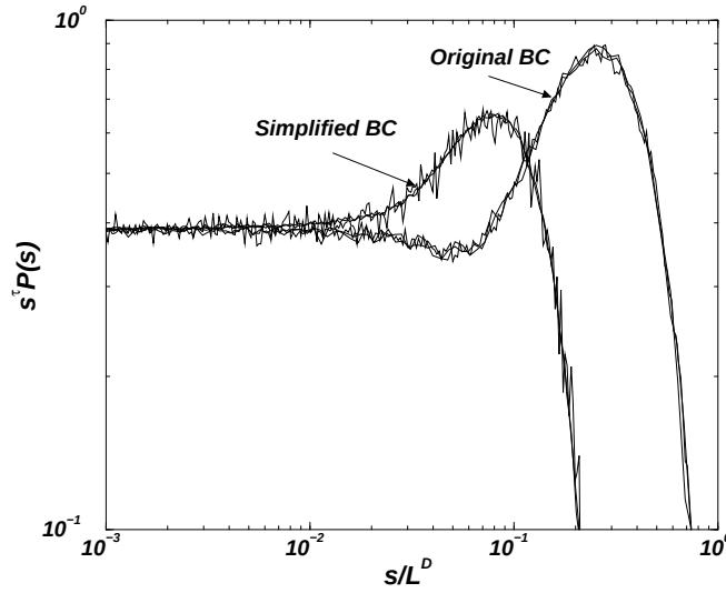
Figure 5.6: Data collapse of binned and rescaled data for the Oslo model with original boundary conditions and with simplified boundaries, focussing on the “bump” of the scaling function. System sizes are L = 640, 1280, 2560 , exponents are \tau = 1.555 \dots and D = 2.25 . There are indeed differences between the two boundary conditions: the most significant is an additional dip in front of the bump in case of the original BC. 8
