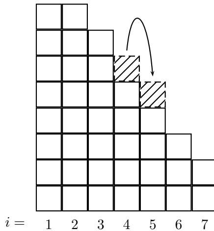
Figure 5.1: A toppling (marked by the arrow) in the Oslo model at site i = 4 transports one grain to the right and changes the slopes according to z_4 \rightarrow z_4 - 2 , z_3 \rightarrow z_3 + 1 and z_5 \rightarrow z_5 + 1 . The toppling grains are shown as dashed and hatched boxes. The process is the same as in the BTW model, see Fig. 1.1, page 37.
