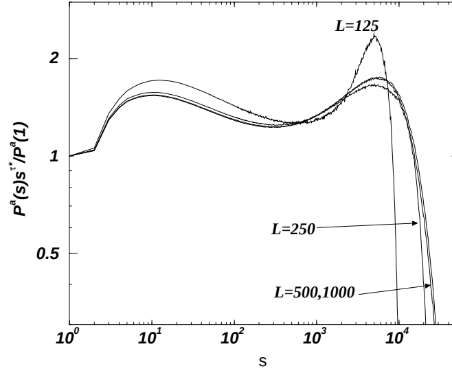
Figure 4.25: Plot of the rescaled PDF \mathcal{P}^a(s; \theta, L) s^{\tau^*} / \mathcal{P}^a(1; \theta, L) for fixed \theta^{-1} = 1000 and different system sizes, L = 125, 250, 500, 1000 . The different shapes make it impossible to collapse the data, as would be expected from a finite size scaling ansatz (4.49) and (4.48).
