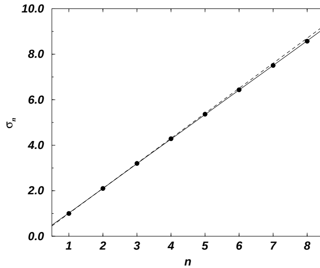
Figure 4.30: Exponents \sigma_n of the scaling of \widetilde{s}^n in \theta vs. n . The slope of this curve gives \lambda and \tau can be derived from the offset. The straight, full line shows the results \lambda = 1.0808\dots and \tau = 2.0506\dots , the dashed line shows \lambda = 1.0998\dots and \tau = 2.0864\dots from a fit excluding \theta^{-1} = 64000 .
