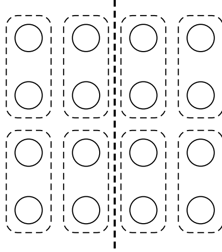
Figure 4.11: If occupied, each site within a dashed box belongs to the same cluster. On a triangular lattice the dashed patches would be triangular, each one containing three sites. The thick dashed line shows the orientation of the boundary between two consecutive slices in the parallelised code, see Sec. 4.2.5.
