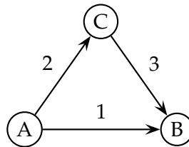
Figure 4.14: Nodes A , B and C send messages in the order indicated. However, it might well happen that the message sent last by node C to node B , namely message 3, arrives at that node before message 1, sent before message 2 was sent, which arrived before message 3 was sent.
