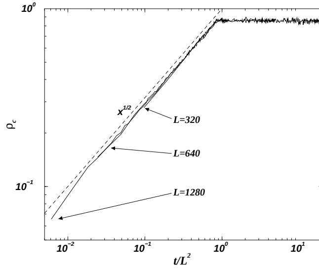
Figure 5.4: A data collapse according to (5.15) for three different system sizes as indicated of the temporal behaviour of the density of susceptible sites ( z_i = z_i^c ) \rho_c(t) in the Oslo model. The time is measured on the macroscopic scale, i.e. it is the number of initial kicks. The dashed line shows \sqrt{x} .
