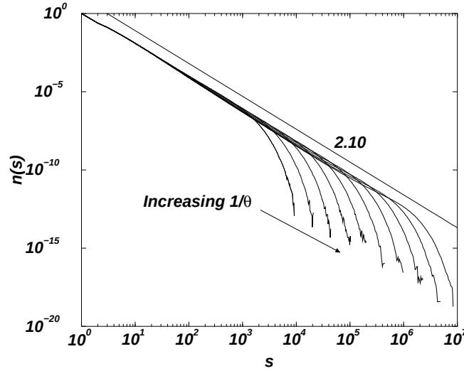
Figure 1.5: The cluster size distribution n(s) of the FFM. The arrow points in the direction of increasing \theta^{-1} , which are from left to right 125, 250, 500, 1000, 2000, 4000, 8000, 16000, 32000 and 64000. The exponent is roughly 2.10, but apparently fits quite well to 2.14 for smaller values of \theta^{-1} .
