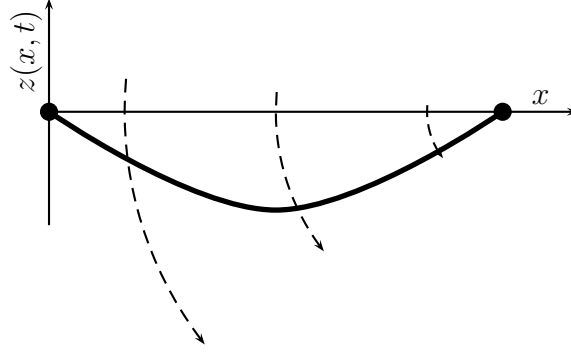
Figure 6.2: Cartoon of an elastic band (thick line) fixed at its two ends (black circles), while the rough background is moving with a velocity linearly increasing from right to left like a cutting disk rotating around x = L , as indicated by the arrows.
