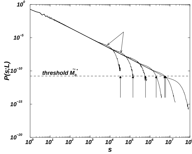
Figure 2.9: Avalanche size distribution \mathcal{P}(s; L) for the Oslo model. System sizes are L = 160, 320, \dots, 5120 . The position of the cutoff is marked by the up-pointing arrows. For small system sizes that technique gives reasonable results, but it fails as soon as the true cutoff becomes too large. Also indicated (two connected arrows) is the small area of an PDF for a smaller system size not covered by the larger one. This area contains all the probability which can be redistributed in the PDF of the larger system sizes.
