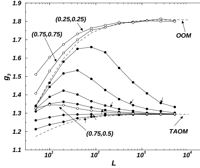
Figure 7.3: Scaling of g_3 [see Eq. (7.4)] for different anisotropies. The filled circles are results for p_r - p_l in the same vertical order as shown in Fig. 7.2 and p_r = 1 . Open circles show other parameters (p_r, p_l) as indicated. The dashed lines are the two extreme cases OOM ( p_r = p_l = 1 ) and the solvable model (TAOM, p_r = 1, p_l = 0 ). The short arrows mark the crossover points in Fig. 7.2.
