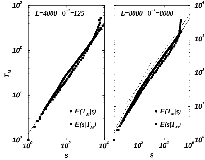
Figure 4.35: E(T_M|s; \theta) and E(s|T_M; \theta) , based on the binned histogram P(s, T_M; \theta) for different values of \theta^{-1} . The straight lines in the plots are 1.4s^{0.615} for \theta^{-1} = 125 (left hand plot) and 1.6s^{0.57} for \theta^{-1} = 8000 . The two dashed lines in the right hand plot show alternative exponents 1/\mu' = 0.7 and 1/\mu' = 0.53 , which are consistent with data either for small values of s or for large values.
