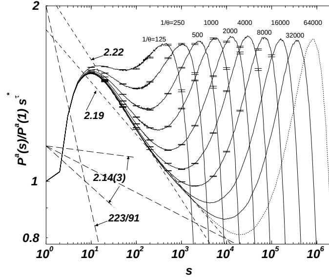
Figure 4.16: The rescaled and binned histogram \frac{P^a(s)}{P^a(1)} s^{\tau^*} , where \tau^* = 2.10 for \theta^{-1} = 125, 250, 500, \dots, 32000, 64000 (as indicated) in a double logarithmic plot. The linear size L is chosen according to the bold printed entries in Tab. 4.3 (page 178) and large enough to ensure absence of finite size effects. The error bars are estimated from shorter runs. The rightmost histogram (dotted, \theta^{-1} = 64000 ) could not be cross-checked by another run, see text. The dashed lines belong to different exponents, whose value is specified as the sum of the slope in the diagram and \tau^* , i.e. a horizontal line would correspond to an exponent 2.1. The shortly dashed lines represent estimated exponents for different regions of the histogram (2.22 for s within approx. [20, 200] and 2.19 for s within [200, 2000] ), the other exponents are from literature, namely 2.14(3) in (Clar et al. , 1994, 1996) and 223/91 \approx 2.45 in (Schenk et al. , 2002). Since it was impossible to relate these exponents to any property of the data, the exact position of the lines associated with them was chosen arbitrarily.
