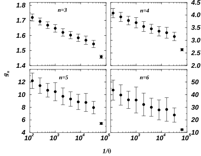
Figure 4.31: The supposedly universal amplitude ratio g_n (4.60) for n = 3, 4, 5, 6 . The error bars are based on a Jackknife scheme (Efron, 1982; Pruessner et al. , 2001) using a roughly estimated correlation time of 50, see Tab. 4.2.
