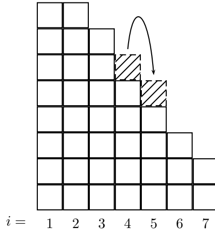
Figure 1.1: A relaxation event in the BTW model. The column of grains at site i - 1 = 4 topples, because its slope ( z_{i-1} = h_{i-1} - h_i ) is above the threshold, here z_4^c = 1 . The toppling grain is shown as a dashed and hatched box. Note that in the next step column i will topple, since it has become unstable, and an avalanche of total size 2 will have formed. Figure drawn after (Jensen, 1998).
