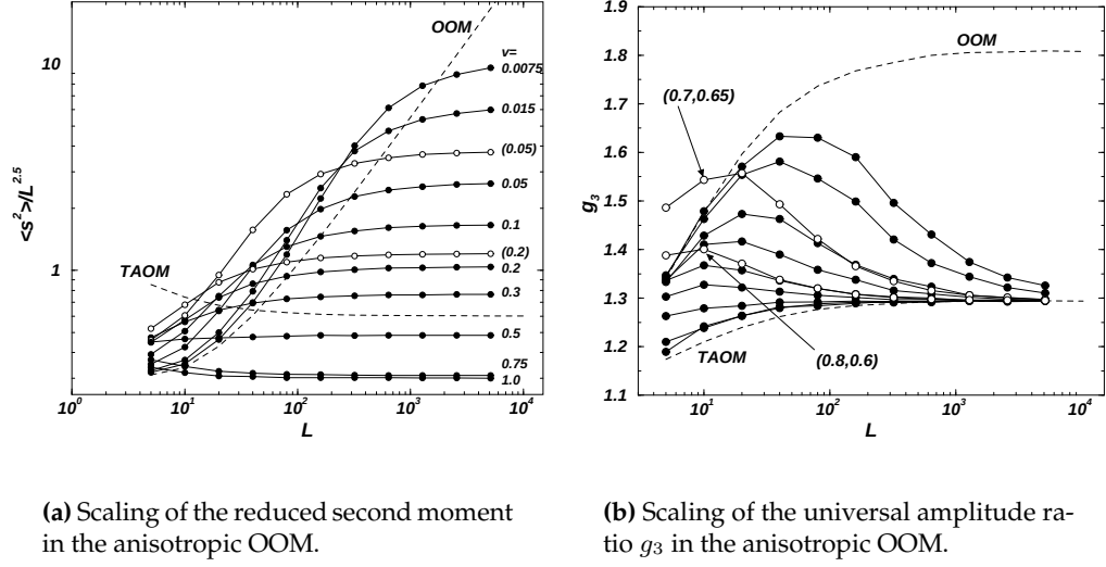
Figure 7.5: Scaling in the anisotropic OOM. Fig. 7.5(a): Rescaled second moment \langle s^2 \rangle / L^{2.5} in the anisotropic OOM versus L for various values of \nu with p_r = 1 (filled circles). For larger \nu the TAOM behaviour sets in much earlier. The dashed lines are the corresponding data of the OOM and the TAOM. The data with opaque circles and \nu = 0.2 (in brackets) is for p_r = 0.8 and p_l = 0.6 . Similar for \nu = 0.05 for p_r = 0.7 and p_l = 0.65 . Fig. 7.5(b): Moment ratio g_3 for different values of \nu (from top to bottom the same order as in Fig. 7.5(a)) in the anisotropic OOM ( p_r = 1 for all filled symbols) and different system sizes L . The upper and the lower dashed lines are the g_3 data of the OOM and the TAOM. For p_r = p_l = 1 the anisotropic OOM is identical to the OOM.
