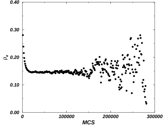
Figure 1.11: An example of the temporal evolution of the density of active sites in directed percolation at p = 0.6435 for a one-dimensional system of size L = 500 . The time is given in Monte Carlo Steps (MCS).
