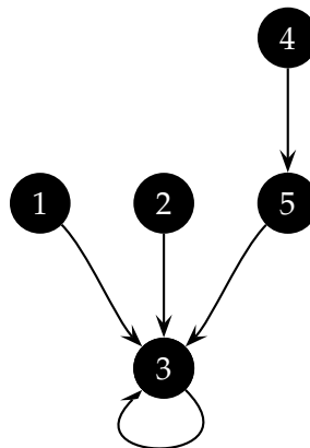
Figure 4.6: The tree-like structure of the largest cluster in Fig. 4.5.
