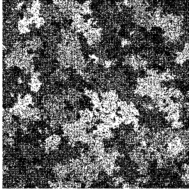
Figure 1.4: The two-dimensional Forest Fire model. Occupied sites are black. The model develops a patchy structure because regions which become completely empty due to the removal of a cluster become homogeneously reforested.
