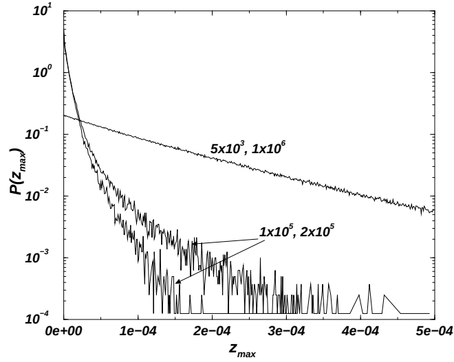
Figure 3.5: The distribution of the maximum \mathcal{P}(z_{\max}) for two different equilibration times and two different initial seeds of the random number generator. System size L = 200 , open boundaries, \alpha = 0.24 . The number of avalanches rejected as transient and accepted as statistics are given in the form “transient, statistics”.
