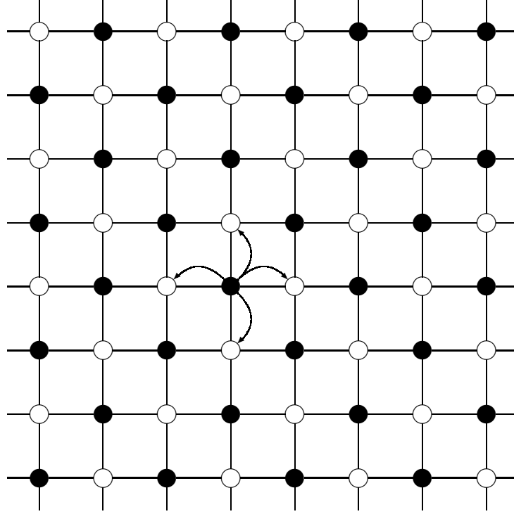
Figure 1.2: The two sub-lattices of a square-lattice, marked by filled and white circles. The set of all nearest neighbours of one sub-lattice is the other one. If only sites on one sub-lattice topple at one time step, only sites on the other will topple in the next one.
