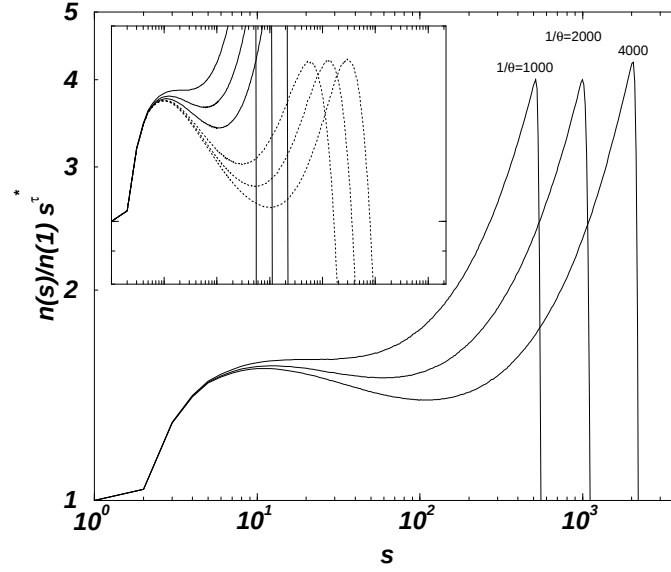
Figure 4.23: The rescaled and binned histogram \bar{n}(s; \theta)s^{\tau^*} (again \tau^* = 2.10 ), for a modified model, where the largest cluster in the system is removed after each driving step, for \theta^{-1} = 1000, 2000, 4000 (as indicated) with linear sizes L = 2000, 2000, 4000 . The inset shows the same data on the scale of Fig. 4.16 for comparison. The data for \theta^{-1} = 1000, 2000, 4000 of the original model as shown in Fig. 4.16 are dotted. The peculiar behaviour of the different height-scaling of the minimum and the maximum is again visible.
