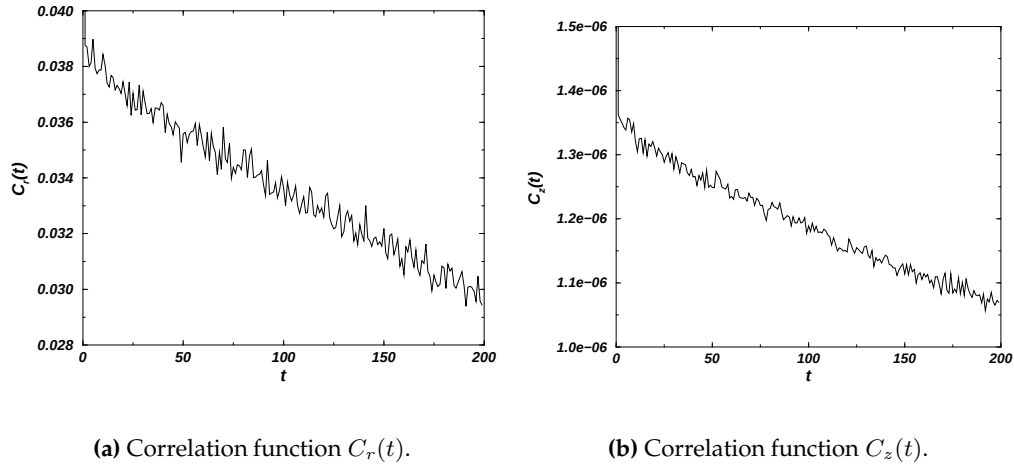
Figure 3.2: Correlation function C_r(t) of the position of the seed of the avalanches and correlation function C_z(t) of the value of the maximum site at time t in the two-dimensional OFC model on a square lattice for L = 256 , open boundaries and \alpha = 0.24 , after 10^6 avalanches, averaged over 3 \times 10^6 avalanches.
