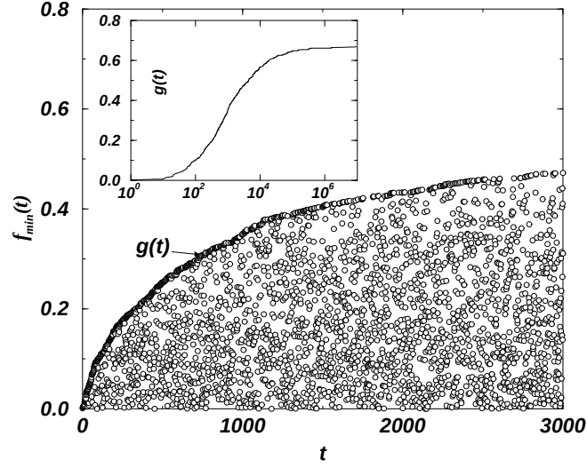
Figure 1.6: The transient behaviour of f_{\min}(t) and g(t) (see text). The thick line is g(t) and consists of dense values of f_{\min}(t) , which changes often but in small steps, because the values of z_i are very dense and if the system gets rid of one small z_i , there is another, only slightly larger value somewhere else in the system. Moreover, f_{\min}(t) decreases for small t only rarely because the probability for an update to arrive below the current g(t) is only g(t) . Dimension is d = 1 and N = 1000 as in Fig. 1.8. The inset shows the long time behaviour of g(t) in a log-linear plot obtained in the same simulation.
