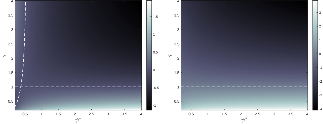
Figure 1: Logarithm of \mathbb{E}(R_j) and \mathbb{V}(R_j) calculated from (27) and (6), showing how the sensitivity to detect model misspecification varies with \varsigma and \psi^* . Dashed lines indicate regions of the parameter space for the true Weibull model where \mathbb{E}(R_j) and \mathbb{V}(R_j) coincide with their putative values under the hypothesised exponential model.
