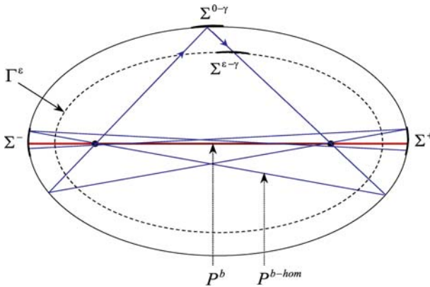
Fig. 9. Billiard trajectory giving rise to a y-symmetric homoclinic orbit (solid)
