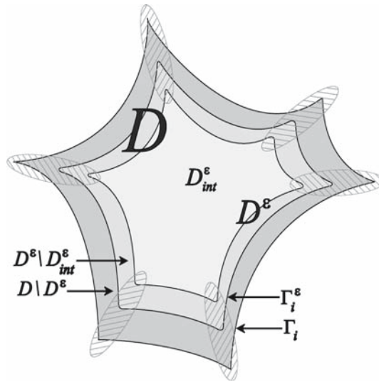
Fig. 6. The partition of the domain D into regions: D^{\epsilon}_{int} \subset D^{\epsilon}
