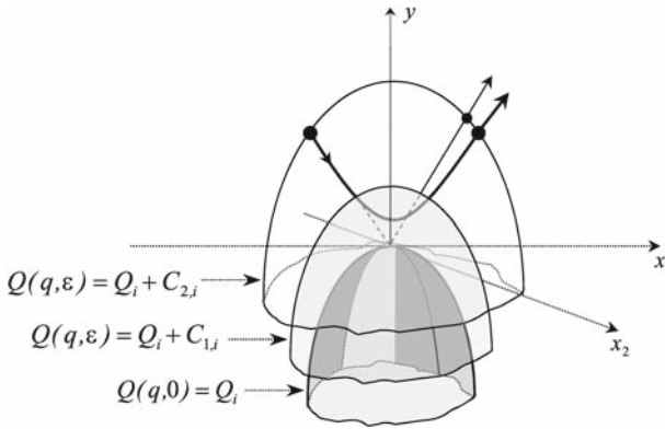
Fig. 2. Level sets of a pattern function Q(q; \epsilon) . A bold line is a trajectory of the Hamiltonian flow near the boundary; a solid is a billiard trajectory
