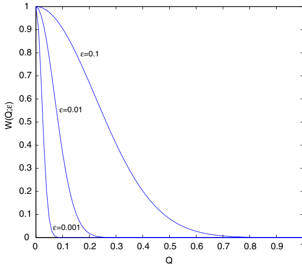
Fig. 3. Gaussian potential given near the boundary by W(Q; \epsilon) = e^{-\frac{Q^2}{\epsilon}} satisfies Conditions I-IV
