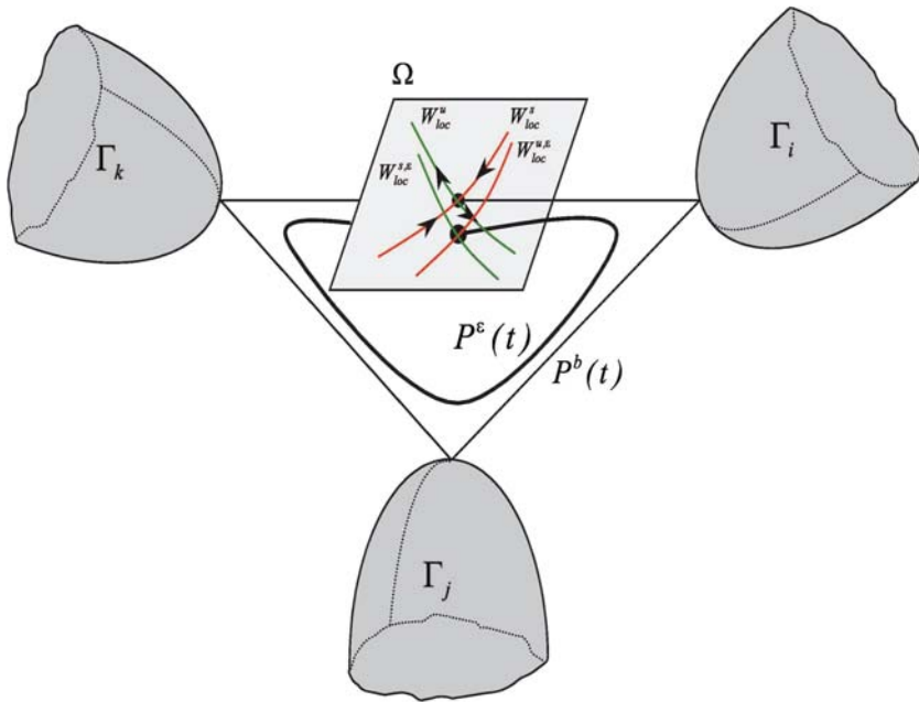
Fig. 8. P^b is a billiard periodic orbit (solid). P^\epsilon is a periodic orbit of the smooth Hamiltonian flow (bold)
