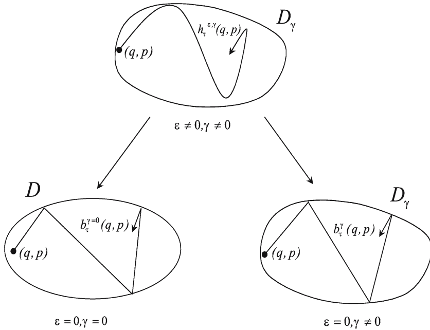
Fig. 10. Perturbation of a billiard flow inside a perturbed ellipsoid family D_\gamma
