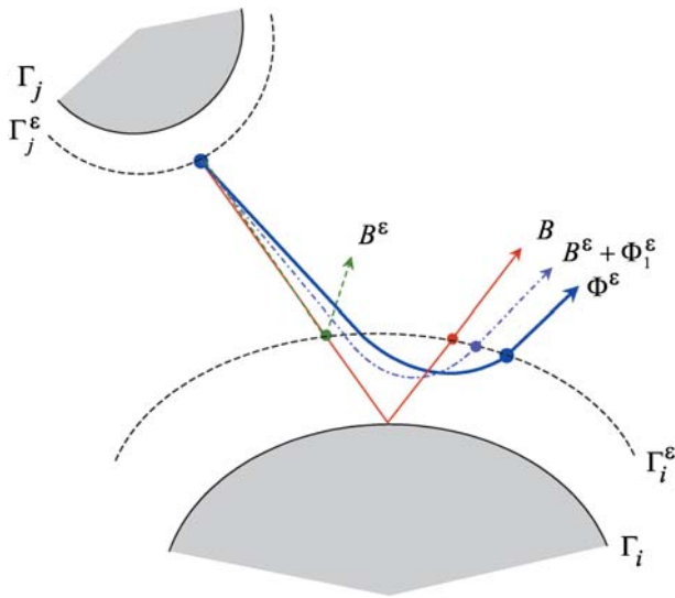
Fig. 7. Billiard map B (solid). Billiard map of the auxiliary billiard B^\epsilon (dashed). Poincaré map for the smooth Hamiltonian flow \Phi^\epsilon (bold). The first approximation of \Phi^\epsilon B^\epsilon + \Phi_1^\epsilon (dash-dotted)
