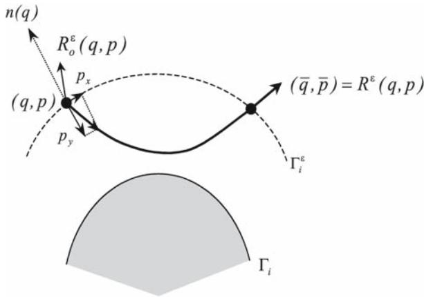
Fig. 5. Reflection from the boundary \Gamma_i . A smooth trajectory is marked by a bold line. An auxiliary billiard trajectory only changes its direction according to the law (25)
