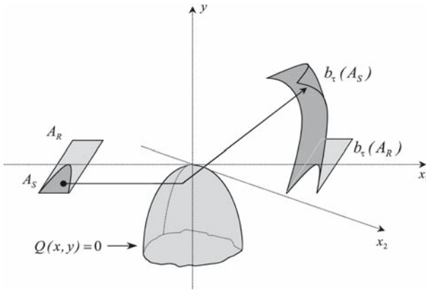
Fig. 1. Singularity near a tangent trajectory. For better visualization we present a slanted hyperplane which is divided into 2 parts: b_t has a square-root singularity on the boundary between A_R and A_S
