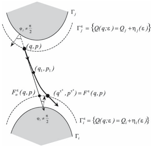
Fig. 4. Free flight between boundaries \Gamma_i^\epsilon and \Gamma_j^\epsilon . A smooth trajectory is marked by a bold line and an auxiliary billiard trajectory is marked by a solid line
