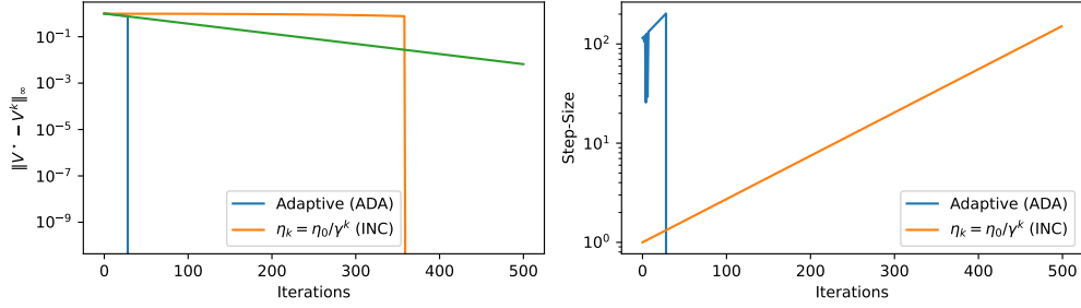
Figure 3: \alpha = 10^{-50} . Green curve: y = \gamma^x .
