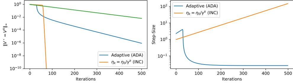
Figure 1: \alpha = 10^{-1} . Green curve: y = \gamma^x .
