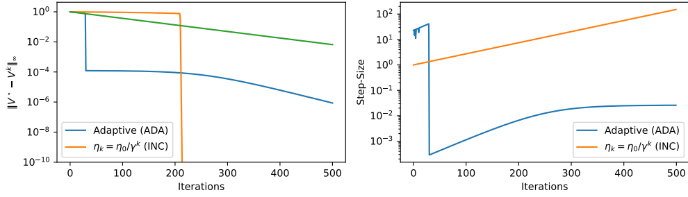
Figure 2: \alpha = 10^{-10} . Green curve: y = \gamma^x .
