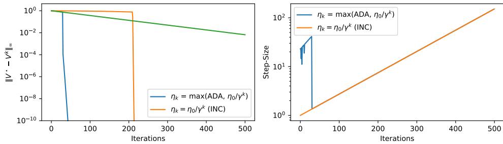
Figure 4: \alpha = 10^{-10} . \eta_k = \max(\text{Adaptive}, \eta_0/\gamma^k) means the step-size is chosen as the largest between our "Adaptive" and the geometrically increasing of [38]. Green curve: y = \gamma^x .
