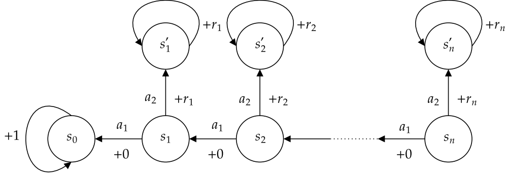
Figure 5: Example MDP used in the proof of Theorem 4.2
